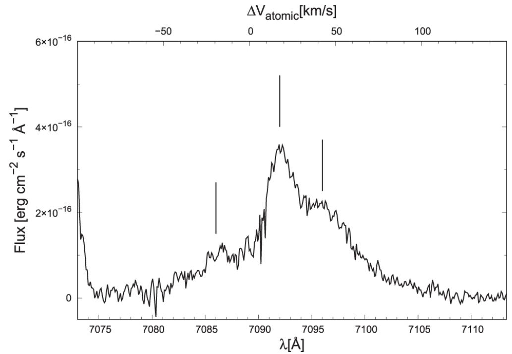
Figure 2. from A PROFILE ANALYSIS OF RAMAN-SCATTERED O VI BANDS AT 6825 AND 7082 IN SANDULEAK'S STAR null 2016 APJ 833 286 doi:10.3847/1538-4357/833/2/286 https://dx.doi.org/10.3847/1538-4357/833/2/286 © 2016. The American Astronomical Society. All rights reserved.
