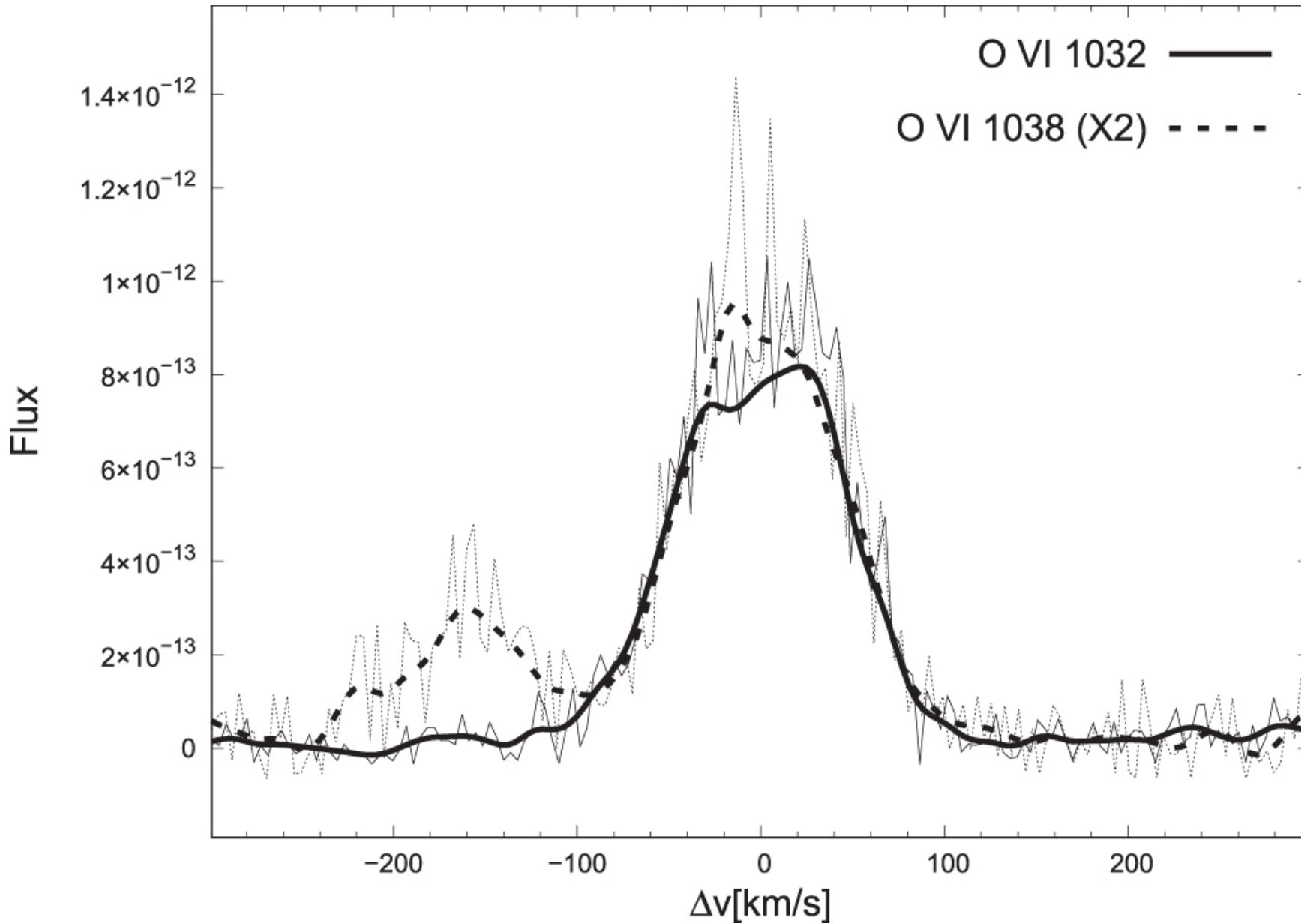
Figure 1. from A PROFILE ANALYSIS OF RAMAN-SCATTERED O VI BANDS AT 6825 AND 7082 IN SANDULEAK'S STAR null 2016 APJ 833 286 doi:10.3847/1538-4357/833/2/286 https://dx.doi.org/10.3847/1538-4357/833/2/286 © 2016. The American Astronomical Society. All rights reserved.
