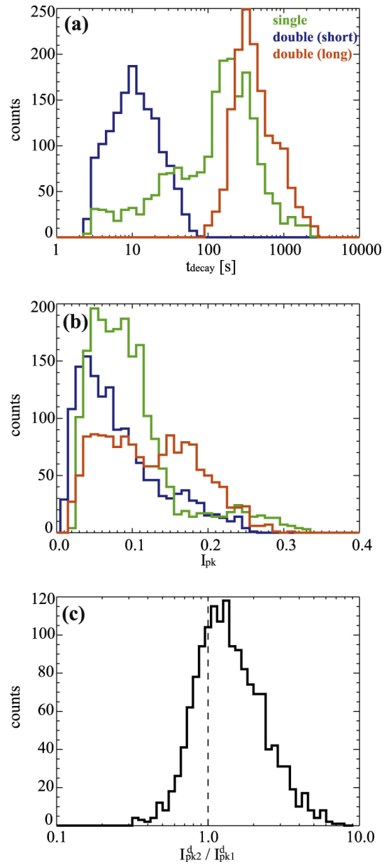
Figure 7. from TEMPORAL EVOLUTION AND SPATIAL DISTRIBUTION OF WHITE-LIGHT FLARE KERNELS IN A SOLAR FLARE null 2016 APJ 833 50 doi:10.3847/1538-4357/833/1/50 https://dx.doi.org/10.3847/1538-4357/833/1/50
