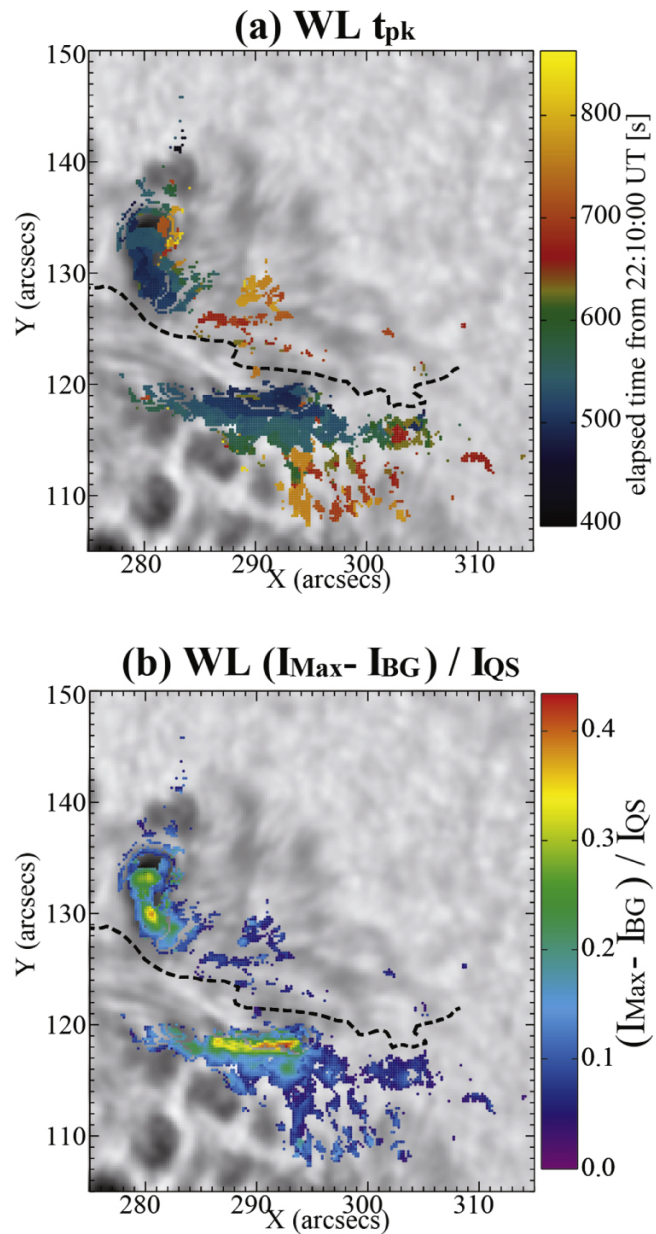
Figure 5. from TEMPORAL EVOLUTION AND SPATIAL DISTRIBUTION OF WHITE-LIGHT FLARE KERNELS IN A SOLAR FLARE null 2016 APJ 833 50 doi:10.3847/1538-4357/833/1/50 https://dx.doi.org/10.3847/1538-4357/833/1/50 © 2016. The American Astronomical Society. All rights reserved.
