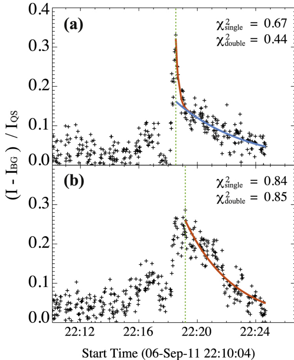
Figure 4. from TEMPORAL EVOLUTION AND SPATIAL DISTRIBUTION OF WHITE-LIGHT FLARE KERNELS IN A SOLAR FLARE null 2016 APJ 833 50 doi:10.3847/1538-4357/833/1/50 https://dx.doi.org/10.3847/1538-4357/833/1/50 © 2016. The American Astronomical Society. All rights reserved.
