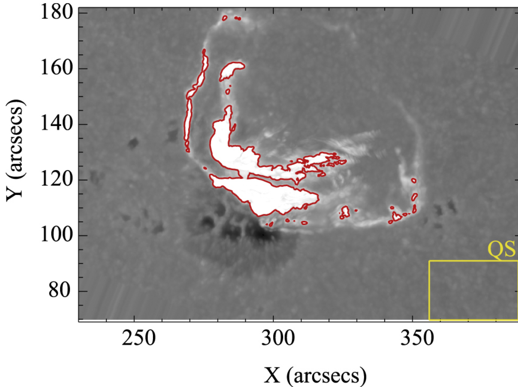
Figure 3. from TEMPORAL EVOLUTION AND SPATIAL DISTRIBUTION OF WHITE-LIGHT FLARE KERNELS IN A SOLAR FLARE null 2016 APJ 833 50 doi:10.3847/1538-4357/833/1/50 https://dx.doi.org/10.3847/1538-4357/833/1/50 © 2016. The American Astronomical Society. All rights reserved.
