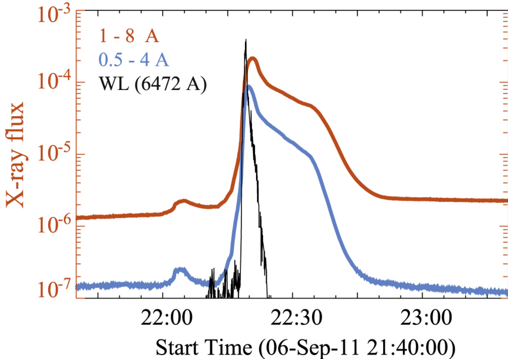
Figure 1. from TEMPORAL EVOLUTION AND SPATIAL DISTRIBUTION OF WHITE-LIGHT FLARE KERNELS IN A SOLAR FLARE null 2016 APJ 833 50 doi:10.3847/1538-4357/833/1/50 https://dx.doi.org/10.3847/1538-4357/833/1/50 © 2016. The American Astronomical Society. All rights reserved.
