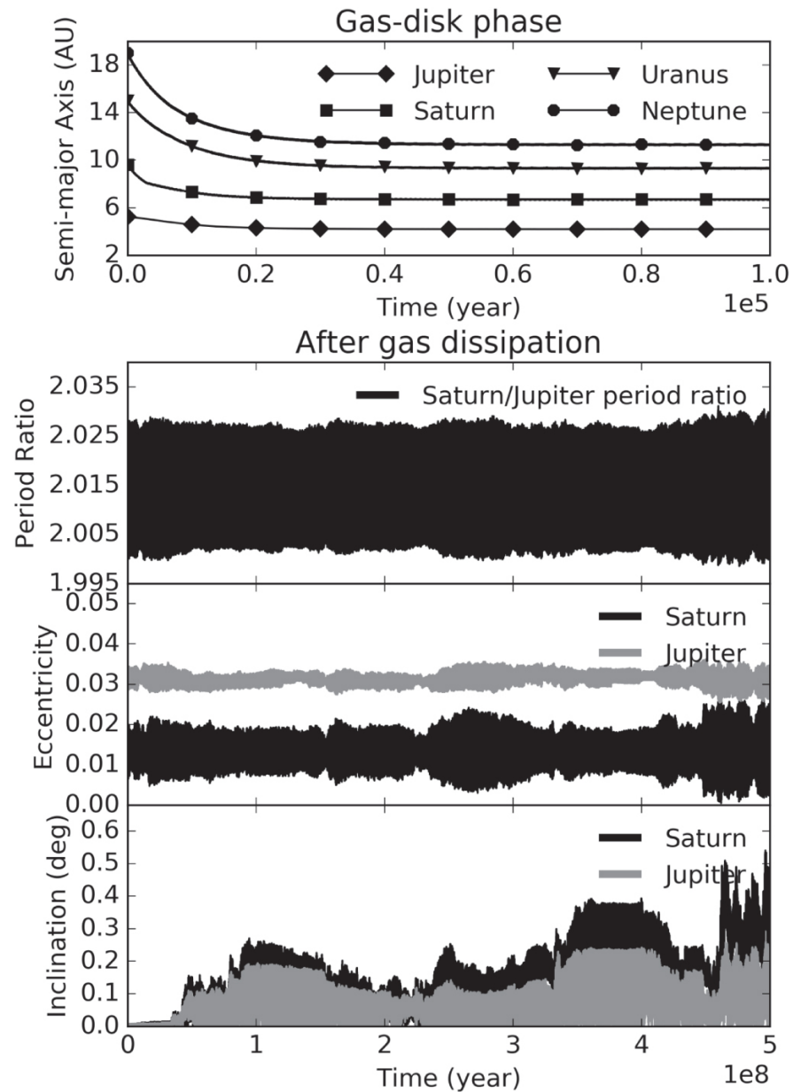
Figure 8. from THE ASTEROID BELT AS A RELIC FROM A CHAOTIC EARLY SOLAR SYSTEM null 2016 APJ 833 40 doi:10.3847/1538-4357/833/1/40 https://dx.doi.org/10.3847/1538-4357/833/1/40 © 2016. The American Astronomical Society. All rights reserved.
