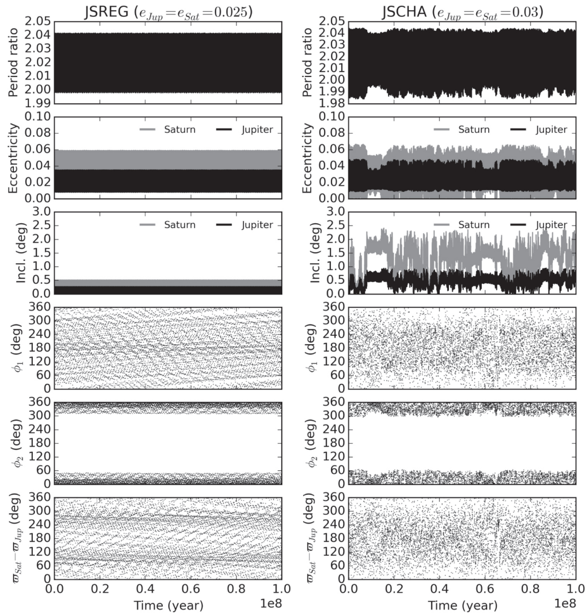
Figure 2. from THE ASTEROID BELT AS A RELIC FROM A CHAOTIC EARLY SOLAR SYSTEM null 2016 APJ 833 40 doi:10.3847/1538-4357/833/1/40 https://dx.doi.org/10.3847/1538-4357/833/1/40
