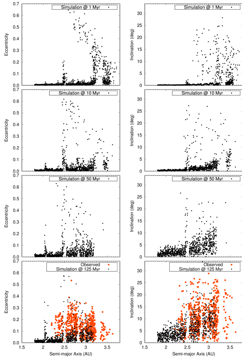
Figure 17. from THE ASTEROID BELT AS A RELIC FROM A CHAOTIC EARLY SOLAR SYSTEM null 2016 APJ 833 40 doi:10.3847/1538-4357/833/1/40 https://dx.doi.org/10.3847/1538-4357/833/1/40
