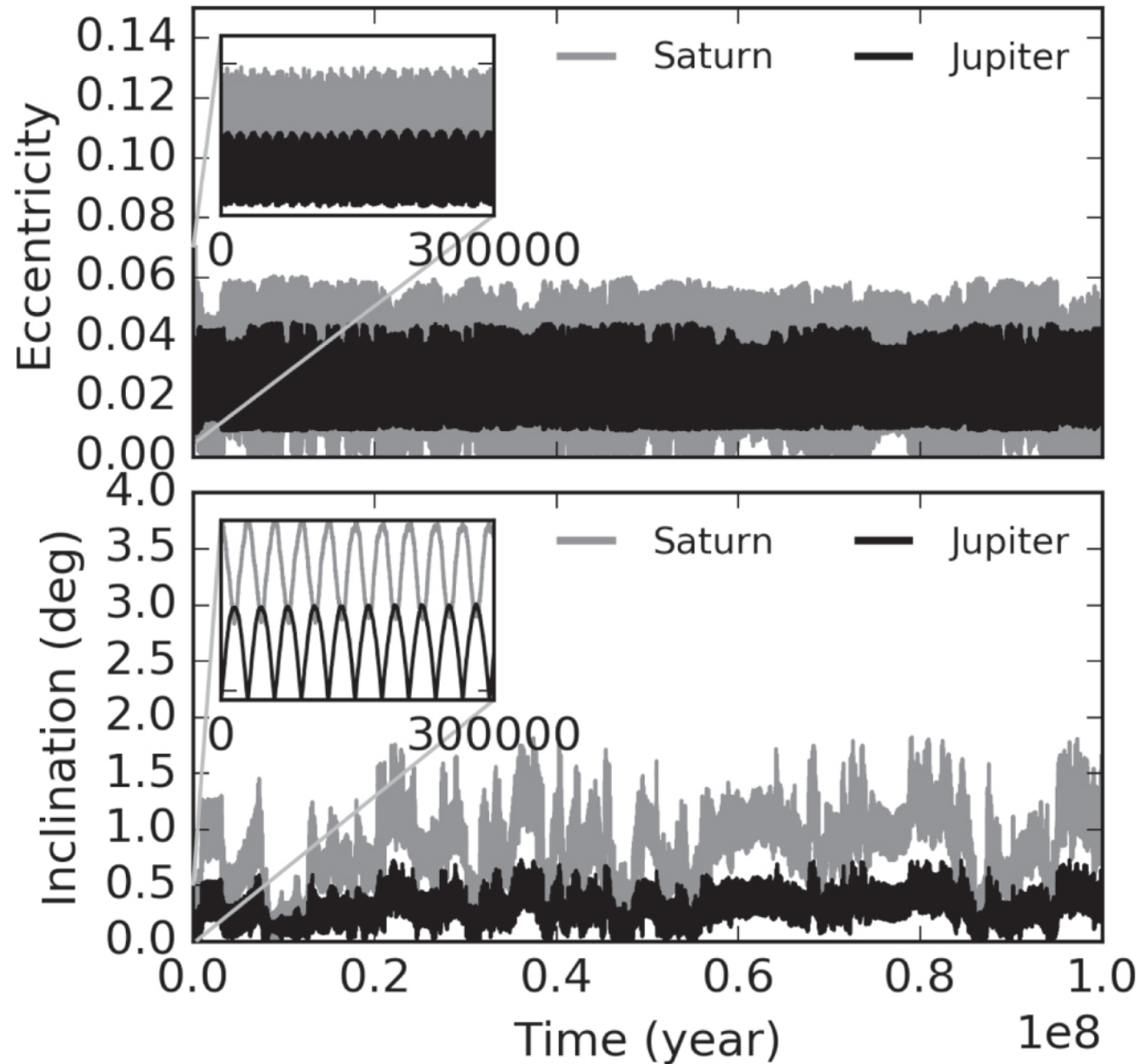
Figure 1. from THE ASTEROID BELT AS A RELIC FROM A CHAOTIC EARLY SOLAR SYSTEM null 2016 APJ 833 40 doi:10.3847/1538-4357/833/1/40 https://dx.doi.org/10.3847/1538-4357/833/1/40 © 2016. The American Astronomical Society. All rights reserved.
