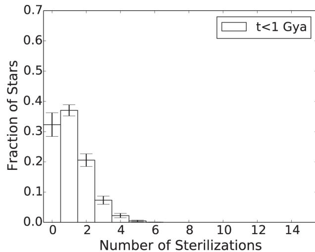
(a) R = 2.5 kpc
