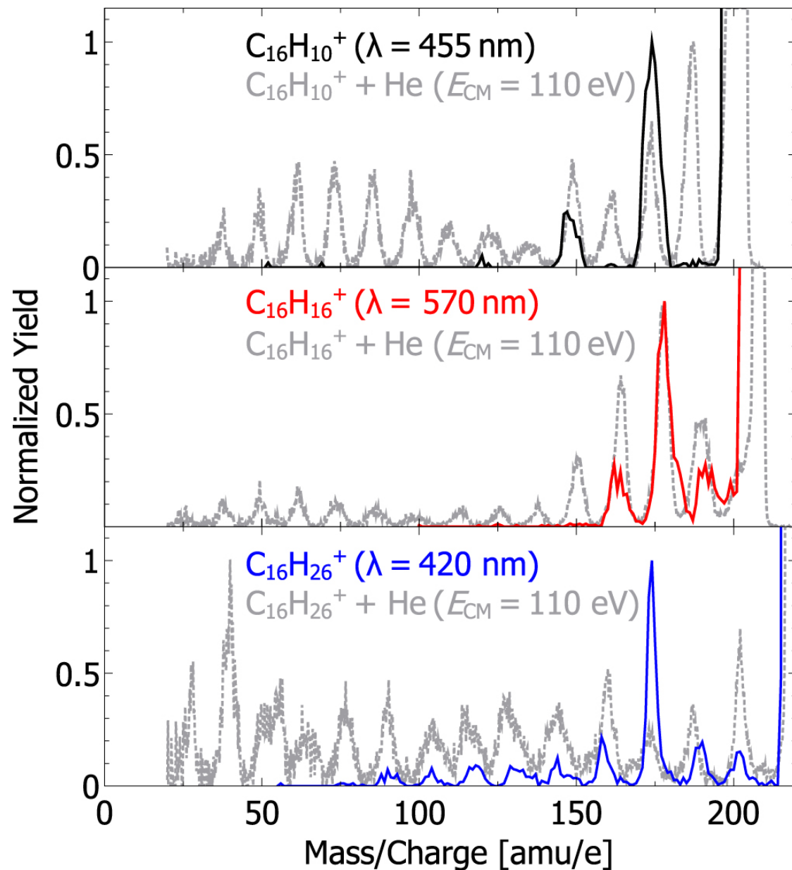
Figure 3. from PHOTO-STABILITY OF SUPER-HYDROGENATED PAHs DETERMINED BY ACTION SPECTROSCOPY EXPERIMENTS null 2016 APJ 832 24 doi:10.3847/0004-637X/832/1/24 https://dx.doi.org/10.3847/0004-637X/832/1/24 © 2016. The American Astronomical Society. All rights reserved.
