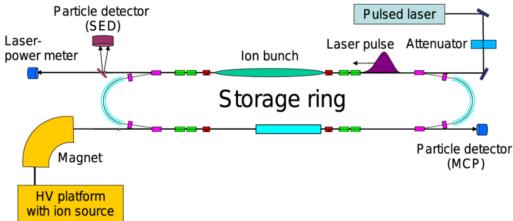
Figure 1. from PHOTO-STABILITY OF SUPER-HYDROGENATED PAHs DETERMINED BY ACTION SPECTROSCOPY EXPERIMENTS null 2016 APJ 832 24 doi:10.3847/0004-637X/832/1/24 https://dx.doi.org/10.3847/0004-637X/832/1/24 © 2016. The American Astronomical Society. All rights reserved.
