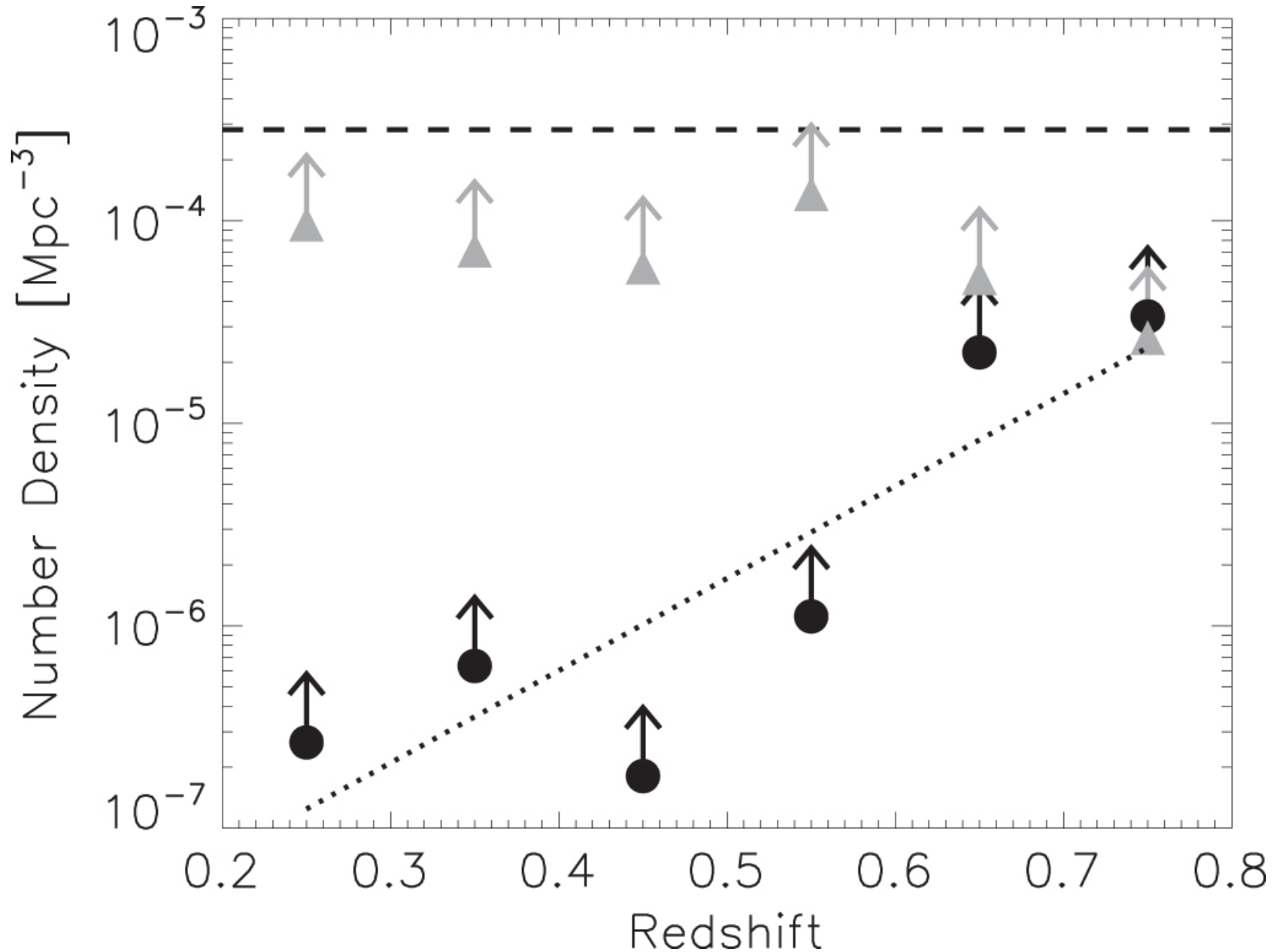
Figure 9. from COMPACT E+A GALAXIES AS A PROGENITOR OF MASSIVE COMPACT QUIESCENT GALAXIES AT 0.2 < z < 0.8 null 2016 APJ 831 146 doi:10.3847/0004-637X/831/2/146 https://dx.doi.org/10.3847/0004-637X/831/2/146 © 2016. The American Astronomical Society. All rights reserved.
