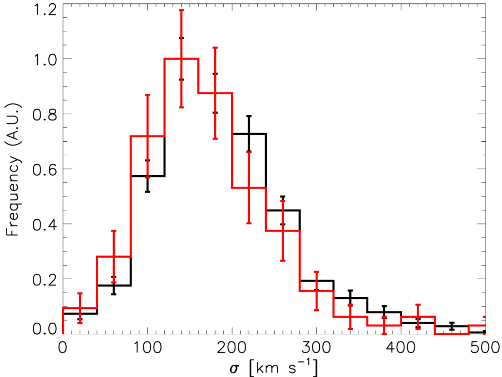
Figure 8. from COMPACT E+A GALAXIES AS A PROGENITOR OF MASSIVE COMPACT QUIESCENT GALAXIES AT 0.2 < z < 0.8 null 2016 APJ 831 146 doi:10.3847/0004-637X/831/2/146 https://dx.doi.org/10.3847/0004-637X/831/2/146 © 2016. The American Astronomical Society. All rights reserved.
