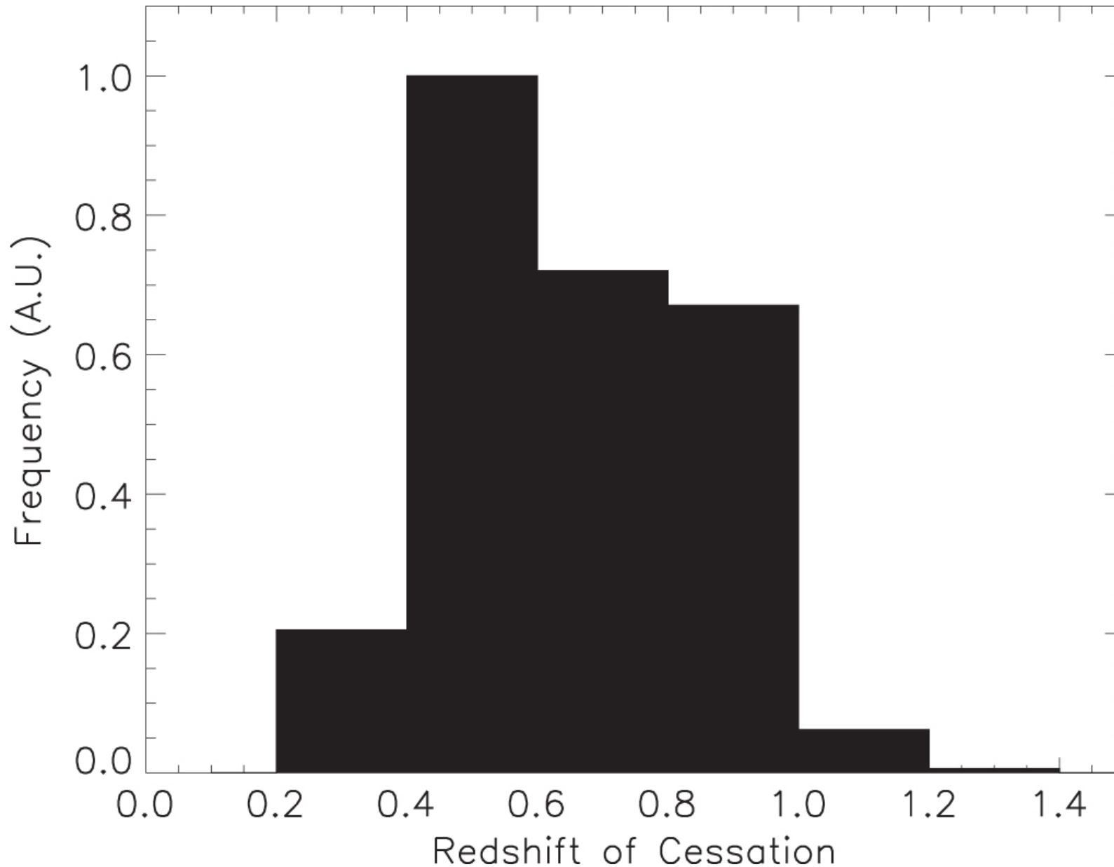
Figure 7. from COMPACT E+A GALAXIES AS A PROGENITOR OF MASSIVE COMPACT QUIESCENT GALAXIES AT 0.2 < z < 0.8 null 2016 APJ 831 146 doi:10.3847/0004-637X/831/2/146 https://dx.doi.org/10.3847/0004-637X/831/2/146 © 2016. The American Astronomical Society. All rights reserved.
