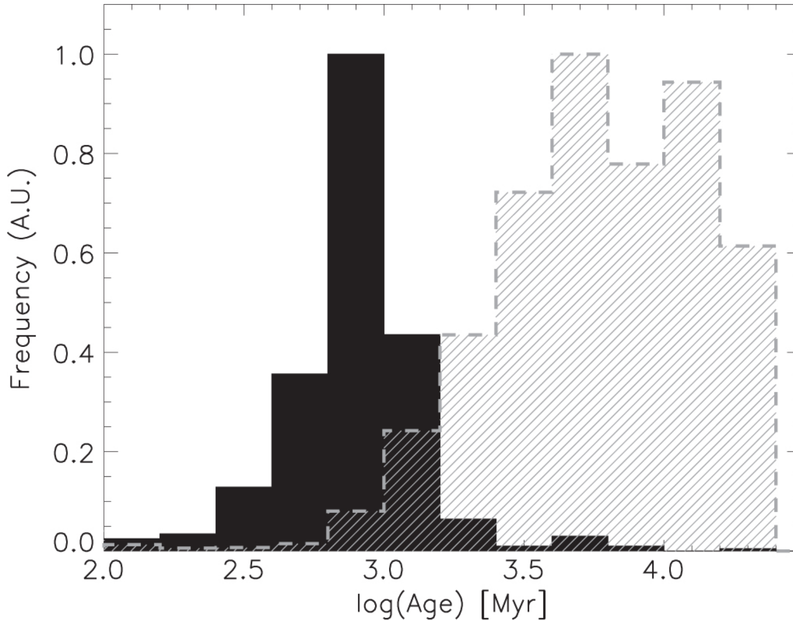
Figure 6. from COMPACT E+A GALAXIES AS A PROGENITOR OF MASSIVE COMPACT QUIESCENT GALAXIES AT 0.2 < z < 0.8 null 2016 APJ 831 146 doi:10.3847/0004-637X/831/2/146 https://dx.doi.org/10.3847/0004-637X/831/2/146 © 2016. The American Astronomical Society. All rights reserved.
