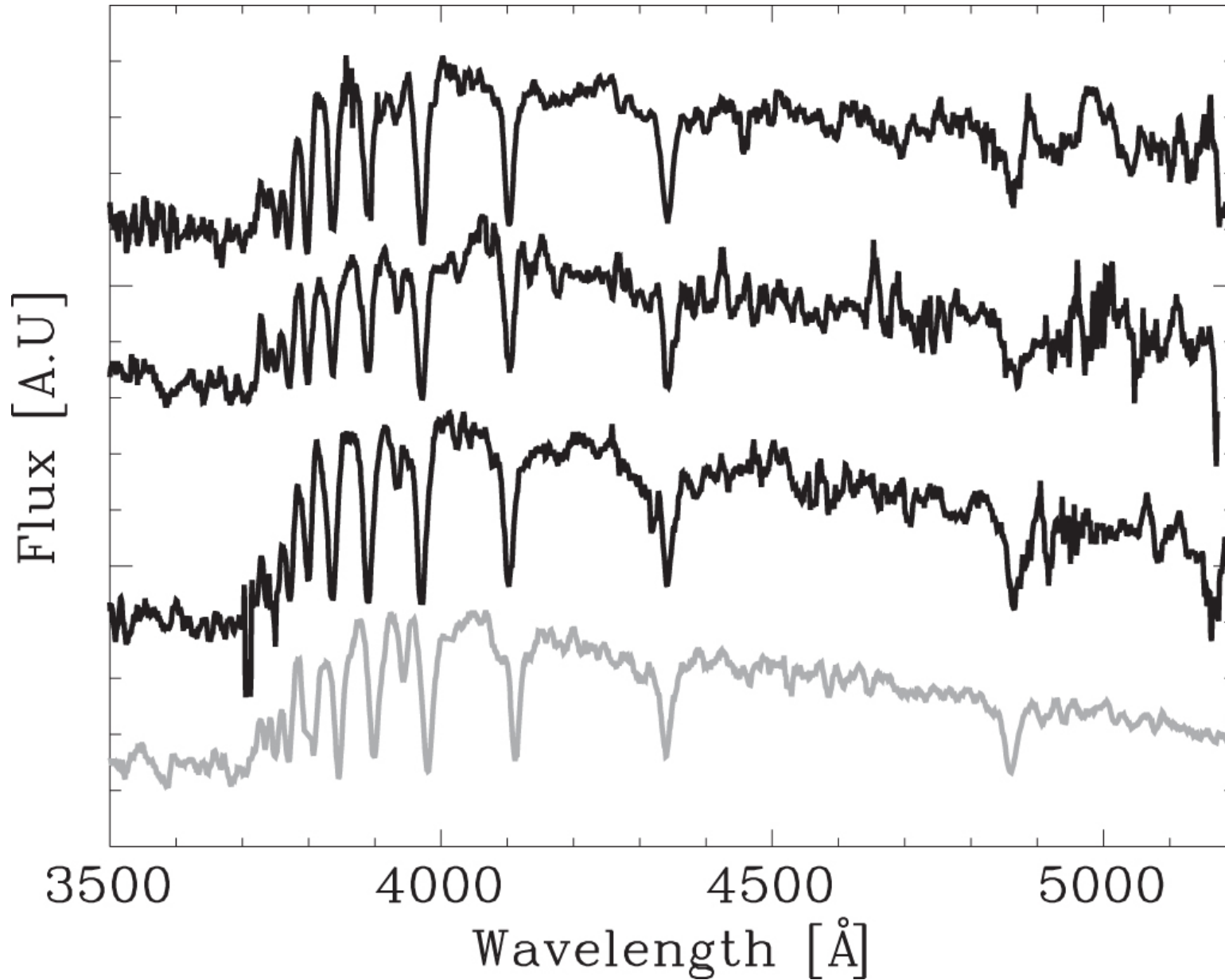
Figure 5. from COMPACT E+A GALAXIES AS A PROGENITOR OF MASSIVE COMPACT QUIESCENT GALAXIES AT 0.2 < z < 0.8 null 2016 APJ 831 146 doi:10.3847/0004-637X/831/2/146 https://dx.doi.org/10.3847/0004-637X/831/2/146 © 2016. The American Astronomical Society. All rights reserved.
