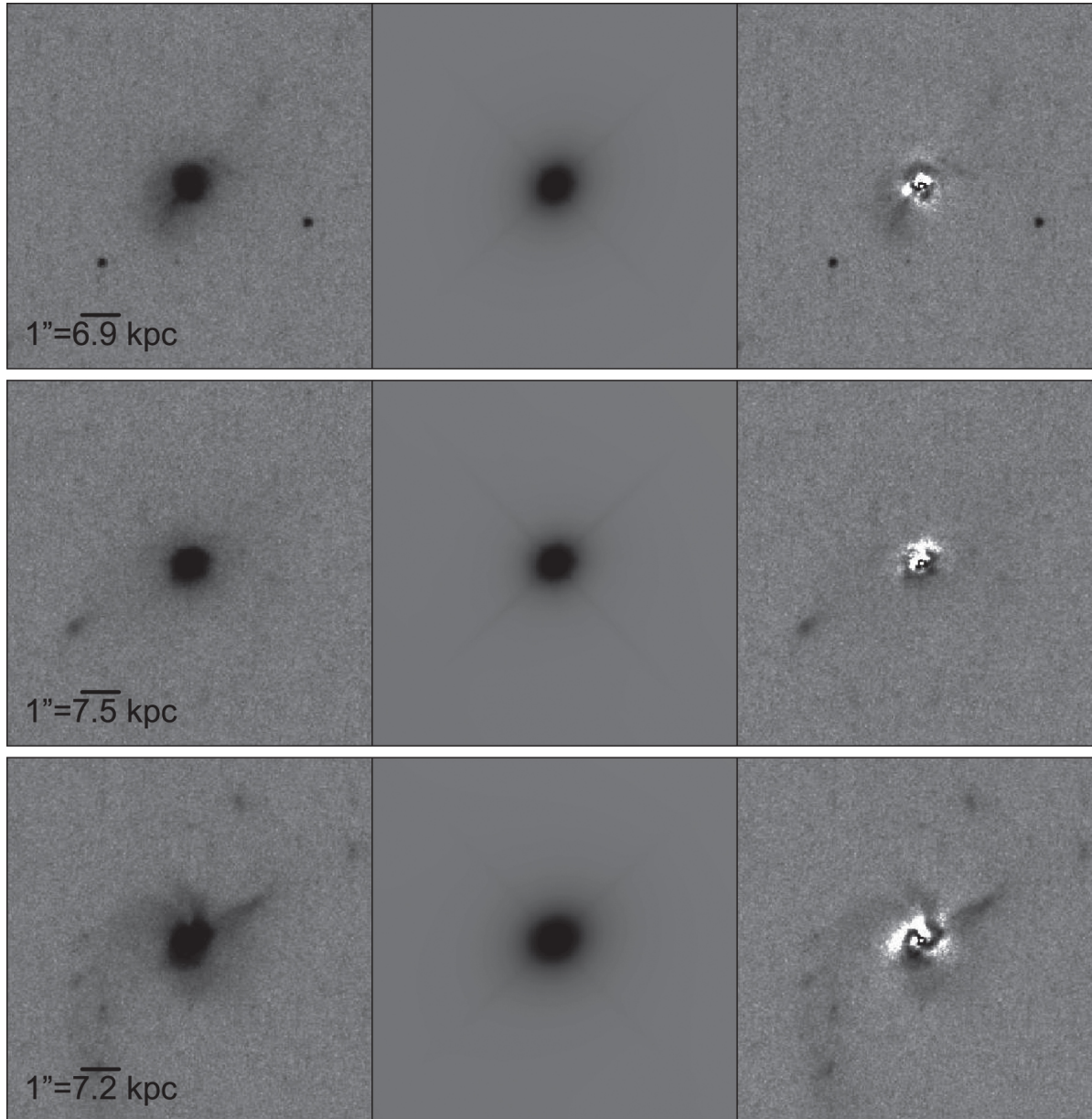
Figure 4. from COMPACT E+A GALAXIES AS A PROGENITOR OF MASSIVE COMPACT QUIESCENT GALAXIES AT 0.2 < z < 0.8 null 2016 APJ 831 146 doi:10.3847/0004-637X/831/2/146 https://dx.doi.org/10.3847/0004-637X/831/2/146 © 2016. The American Astronomical Society. All rights reserved.
