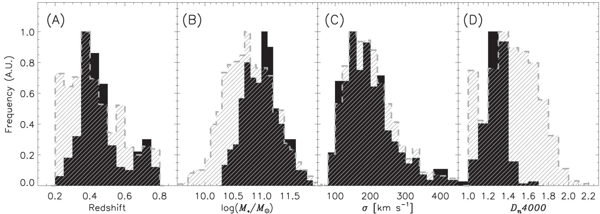
Figure 3. from COMPACT E+A GALAXIES AS A PROGENITOR OF MASSIVE COMPACT QUIESCENT GALAXIES AT 0.2 < z < 0.8 null 2016 APJ 831 146 doi:10.3847/0004-637X/831/2/146 https://dx.doi.org/10.3847/0004-637X/831/2/146 © 2016. The American Astronomical Society. All rights reserved.
