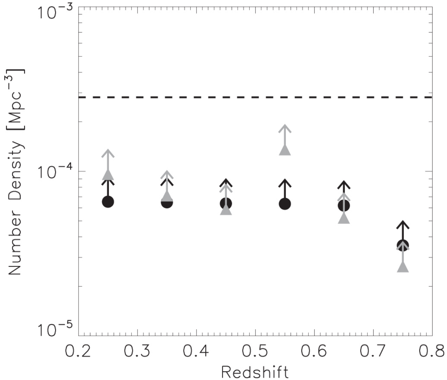
Figure 12. from COMPACT E+A GALAXIES AS A PROGENITOR OF MASSIVE COMPACT QUIESCENT GALAXIES AT 0.2 < z < 0.8 null 2016 APJ 831 146 doi:10.3847/0004-637X/831/2/146 https://dx.doi.org/10.3847/0004-637X/831/2/146 © 2016. The American Astronomical Society. All rights reserved.
