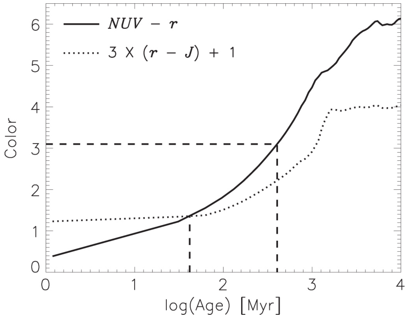
Figure 11. from COMPACT E+A GALAXIES AS A PROGENITOR OF MASSIVE COMPACT QUIESCENT GALAXIES AT 0.2 < z < 0.8 null 2016 APJ 831 146 doi:10.3847/0004-637X/831/2/146 https://dx.doi.org/10.3847/0004-637X/831/2/146 © 2016. The American Astronomical Society. All rights reserved.
