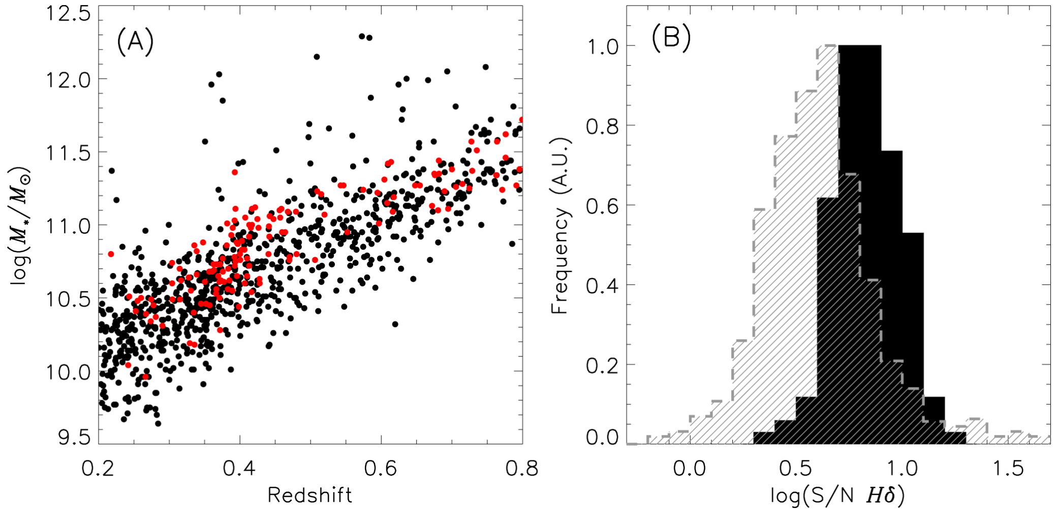
Figure 10. from COMPACT E+A GALAXIES AS A PROGENITOR OF MASSIVE COMPACT QUIESCENT GALAXIES AT 0.2 < z < 0.8 null 2016 APJ 831 146 doi:10.3847/0004-637X/831/2/146 https://dx.doi.org/10.3847/0004-637X/831/2/146 © 2016. The American Astronomical Society. All rights reserved.
