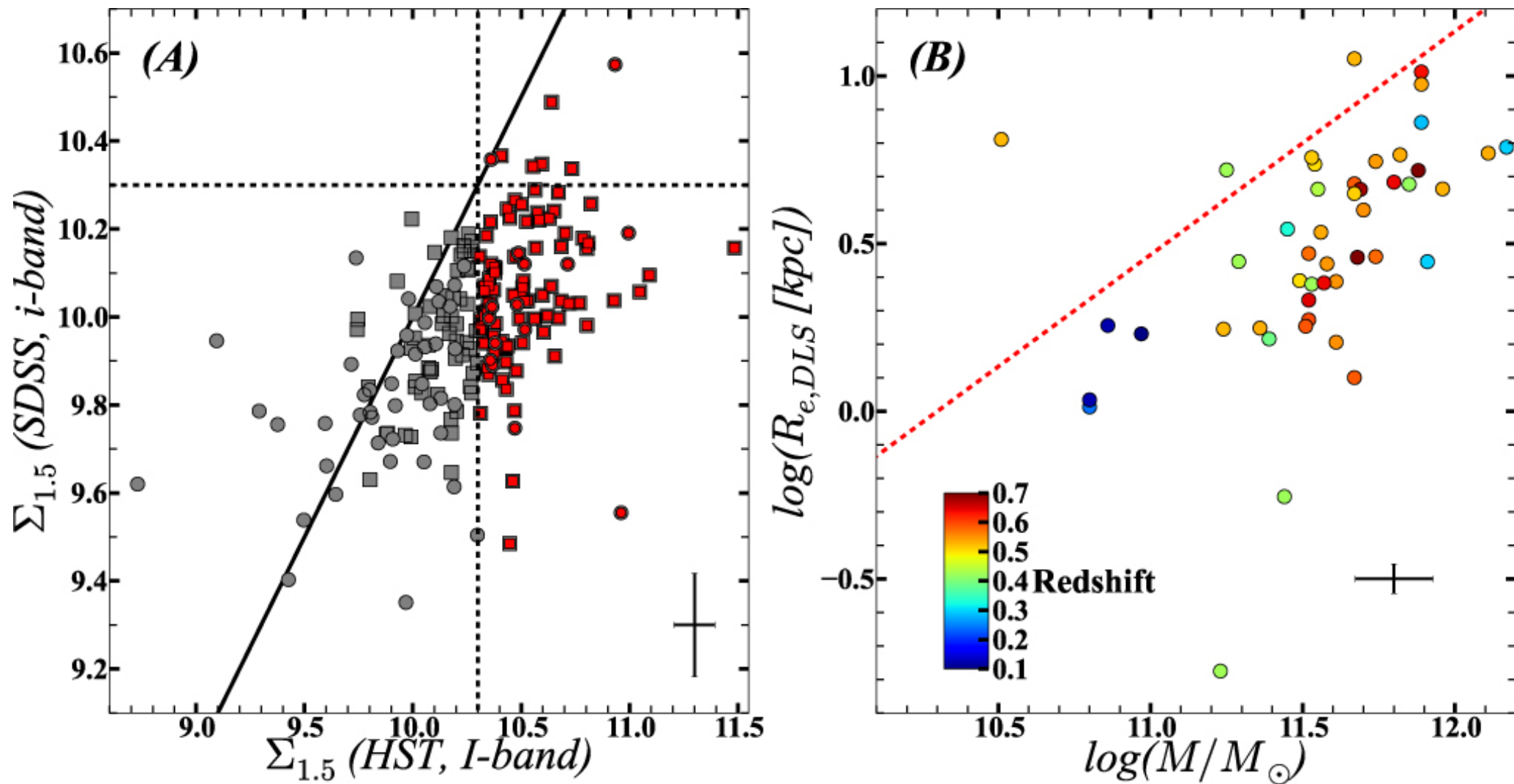
Figure 1. from COMPACT E+A GALAXIES AS A PROGENITOR OF MASSIVE COMPACT QUIESCENT GALAXIES AT 0.2 < z < 0.8 null 2016 APJ 831 146 doi:10.3847/0004-637X/831/2/146 https://dx.doi.org/10.3847/0004-637X/831/2/146 © 2016. The American Astronomical Society. All rights reserved.
