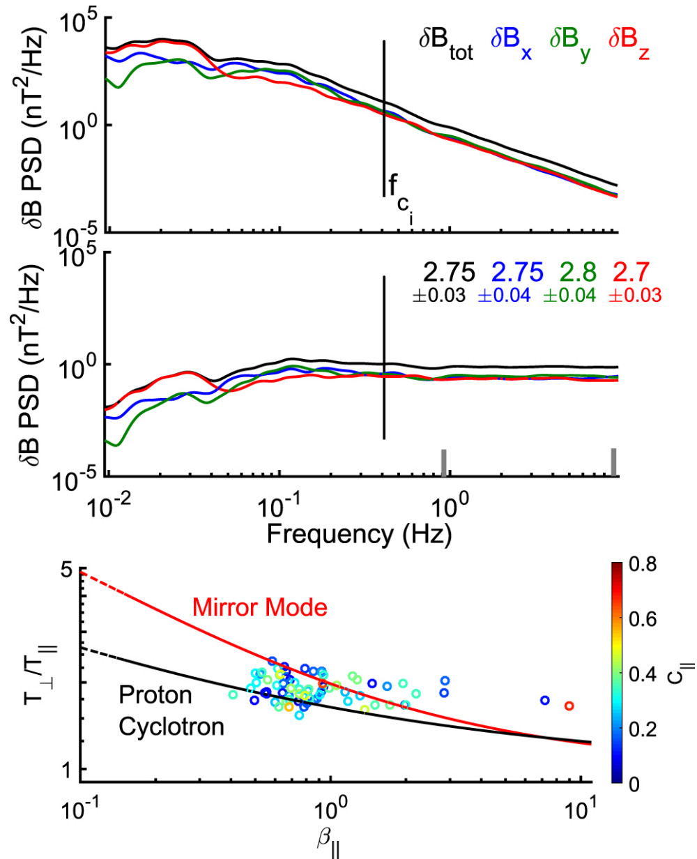
Figure 5. from THE EFFECTS OF KINETIC INSTABILITIES ON SMALL-SCALE TURBULENCE IN EARTH'S MAGNETOSHEATH null 2016 APJ 829 54 doi:10.3847/0004-637X/829/1/54 https://dx.doi.org/10.3847/0004-637X/829/1/54 © 2016. The American Astronomical Society. All rights reserved.
