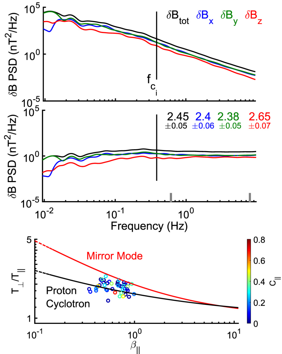
Figure 4. from THE EFFECTS OF KINETIC INSTABILITIES ON SMALL-SCALE TURBULENCE IN EARTH'S MAGNETOSHEATH null 2016 APJ 829 54 doi:10.3847/0004-637X/829/1/54 https://dx.doi.org/10.3847/0004-637X/829/1/54 © 2016. The American Astronomical Society. All rights reserved.
