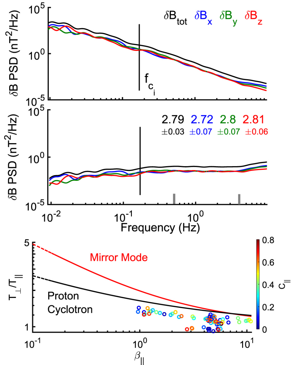
Figure 2. from THE EFFECTS OF KINETIC INSTABILITIES ON SMALL-SCALE TURBULENCE IN EARTH'S MAGNETOSHEATH null 2016 APJ 829 54 doi:10.3847/0004-637X/829/1/54 https://dx.doi.org/10.3847/0004-637X/829/1/54
