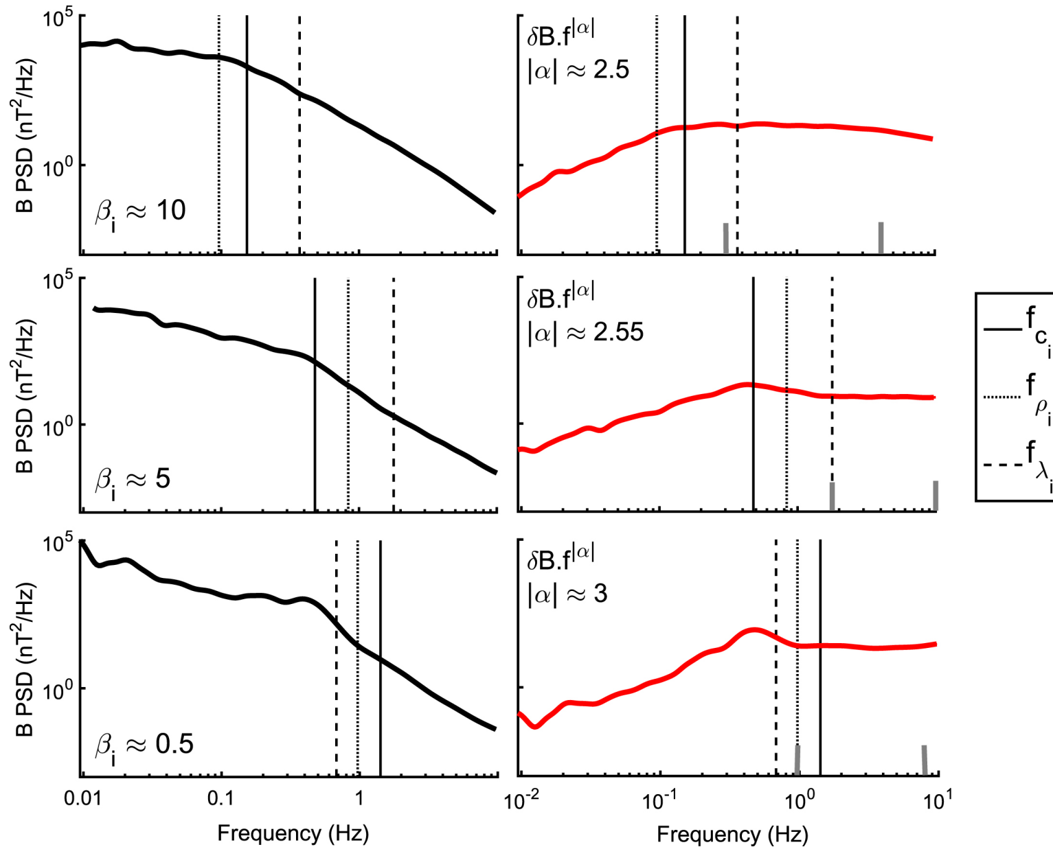
Figure 1. from THE EFFECTS OF KINETIC INSTABILITIES ON SMALL-SCALE TURBULENCE IN EARTH'S MAGNETOSHEATH null 2016 APJ 829 54 doi:10.3847/0004-637X/829/1/54 https://dx.doi.org/10.3847/0004-637X/829/1/54 © 2016. The American Astronomical Society. All rights reserved.
