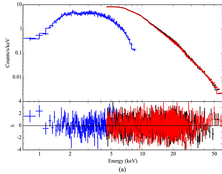
Figure 5. from A NuSTAR OBSERVATION OF THE REFLECTION SPECTRUM OF THE LOW-MASS X-RAY BINARY 4U 1728-34 null 2016 APJ 827 134 doi:10.3847/0004-637X/827/2/134 https://dx.doi.org/10.3847/0004-637X/827/2/134 © 2016. The American Astronomical Society. All rights reserved.
