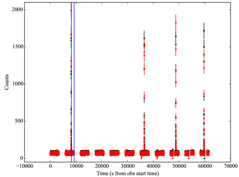
Figure 2. from A NuSTAR OBSERVATION OF THE REFLECTION SPECTRUM OF THE LOW-MASS X-RAY BINARY 4U 1728-34 null 2016 APJ 827 134 doi:10.3847/0004-637X/827/2/134 https://dx.doi.org/10.3847/0004-637X/827/2/134 © 2016. The American Astronomical Society. All rights reserved.
