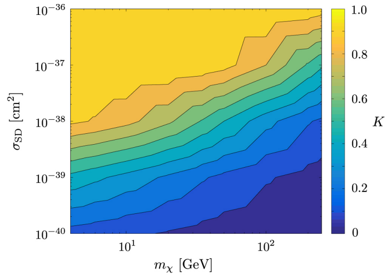
(a) Spin dependent
