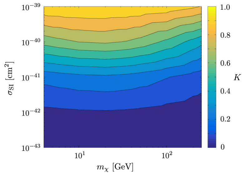
(b) Spin independent
