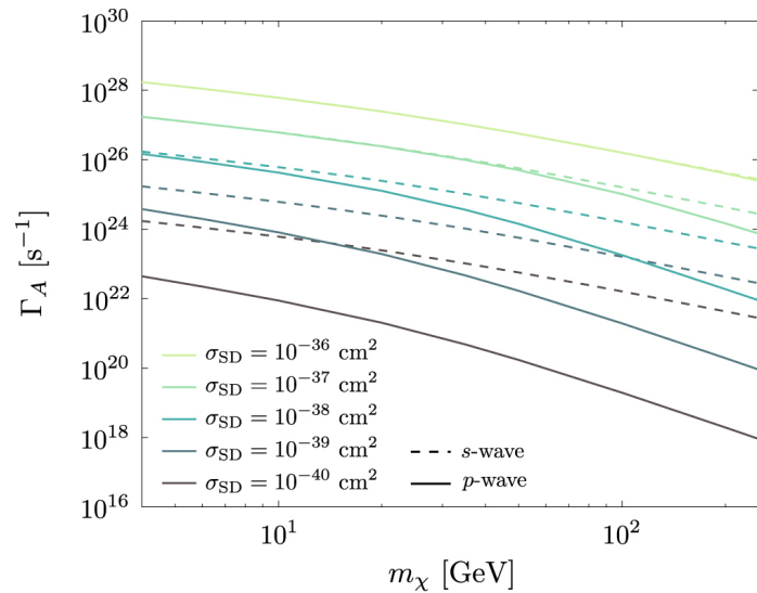
(a) Spin dependent
