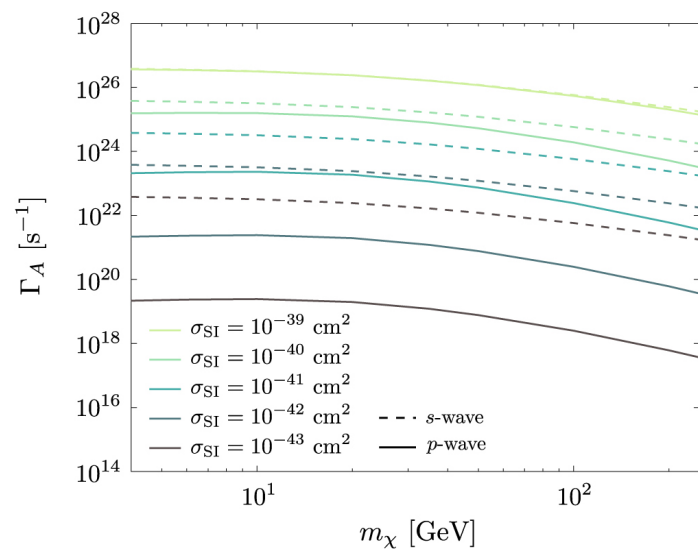
(b) Spin independent
