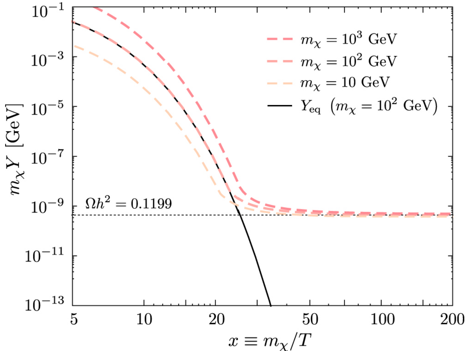
Figure 1. from NEW LIMITS ON THERMALLY ANNIHILATING DARK MATTER FROM NEUTRINO TELESCOPES null 2016 APJ 827 130 doi:10.3847/0004-637X/827/2/130 https://dx.doi.org/10.3847/0004-637X/827/2/130 © 2016. The American Astronomical Society. All rights reserved.
