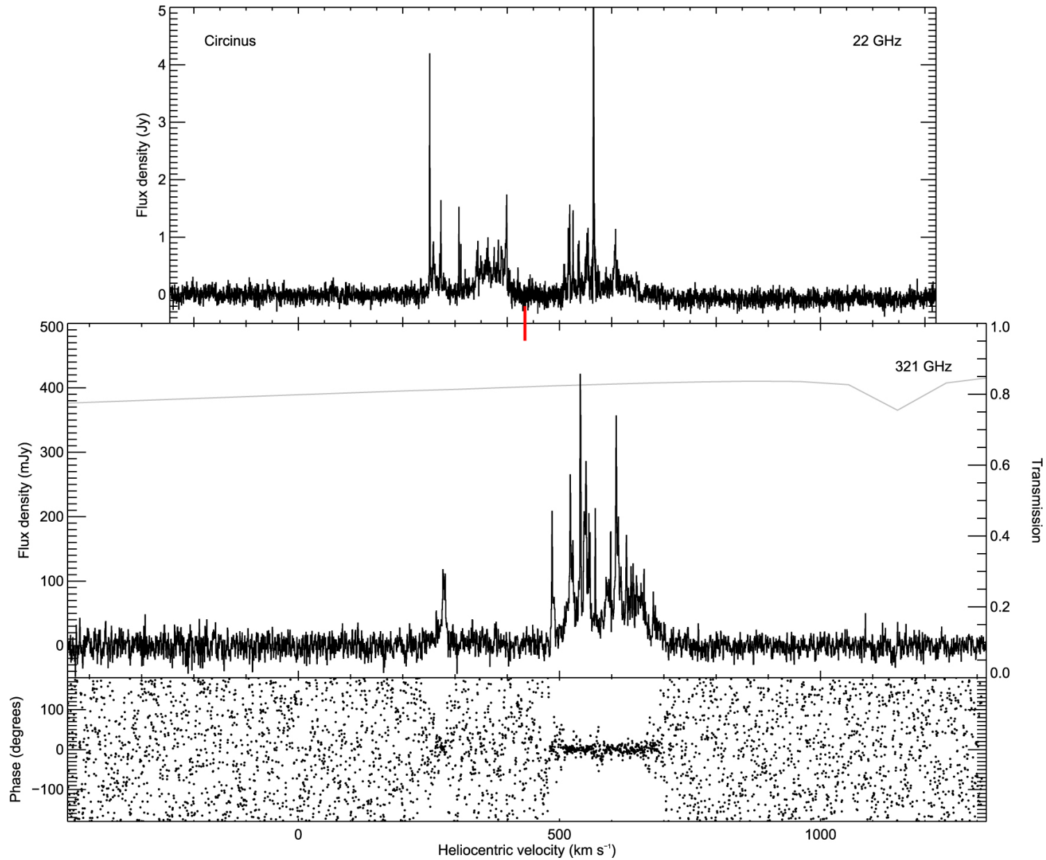
Figure 2. from SUBMILLIMETER H 2 O MEGAMASERS IN NGC 4945 AND THE CIRCINUS GALAXY null 2016 APJ 827 68 doi:10.3847/0004-637X/827/1/68 https://dx.doi.org/10.3847/0004-637X/827/1/68 © 2016. The American Astronomical Society. All rights reserved.
