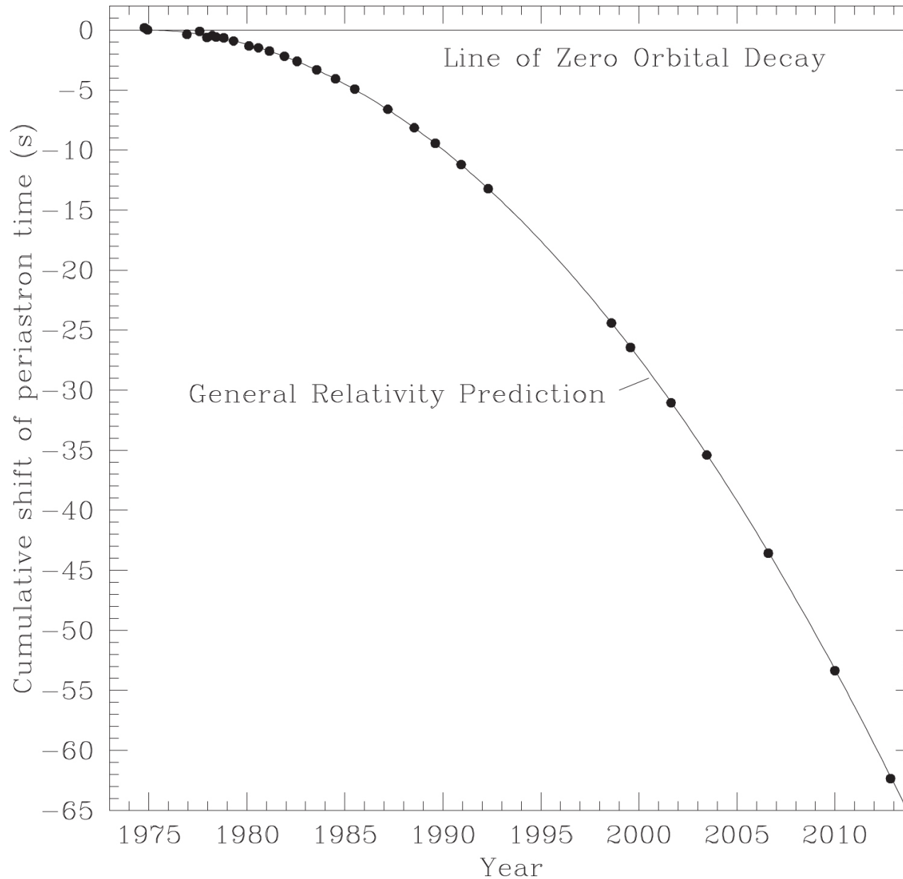
Figure 3. from RELATIVISTIC MEASUREMENTS FROM TIMING THE BINARY PULSAR PSR B1913+16 null 2016 APJ 829 55 doi:10.3847/0004-637X/829/1/55 https://dx.doi.org/10.3847/0004-637X/829/1/55 © 2016. The American Astronomical Society. All rights reserved.
