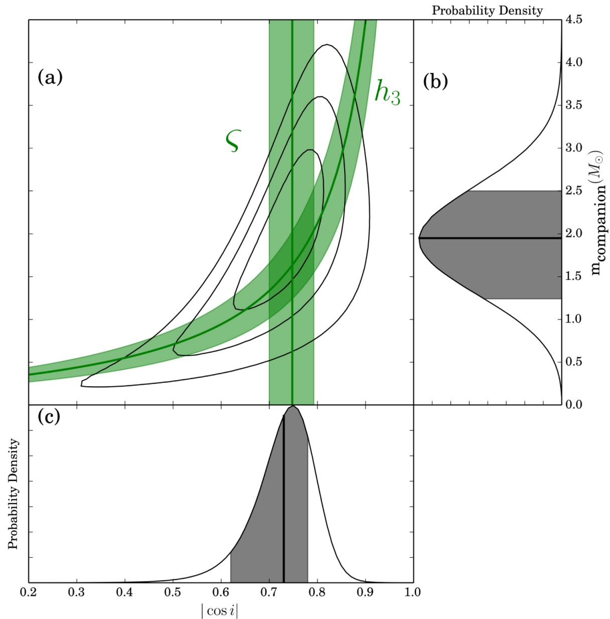
Figure 2. from RELATIVISTIC MEASUREMENTS FROM TIMING THE BINARY PULSAR PSR B1913+16 null 2016 APJ 829 55 doi:10.3847/0004-637X/829/1/55 https://dx.doi.org/10.3847/0004-637X/829/1/55 © 2016. The American Astronomical Society. All rights reserved.
