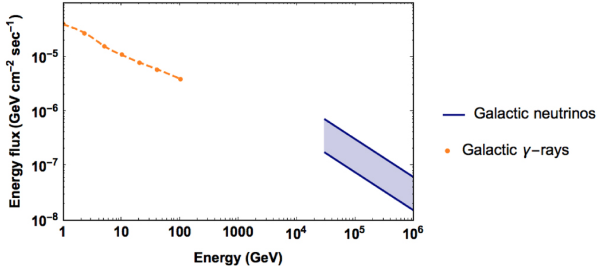
Figure 8. from EXTRAGALACTIC PLUS GALACTIC MODEL FOR ICECUBE NEUTRINO EVENTS null 2016 APJ 826 185 doi:10.3847/0004-637X/826/2/185 https://dx.doi.org/10.3847/0004-637X/826/2/185 © 2016. The American Astronomical Society. All rights reserved.
