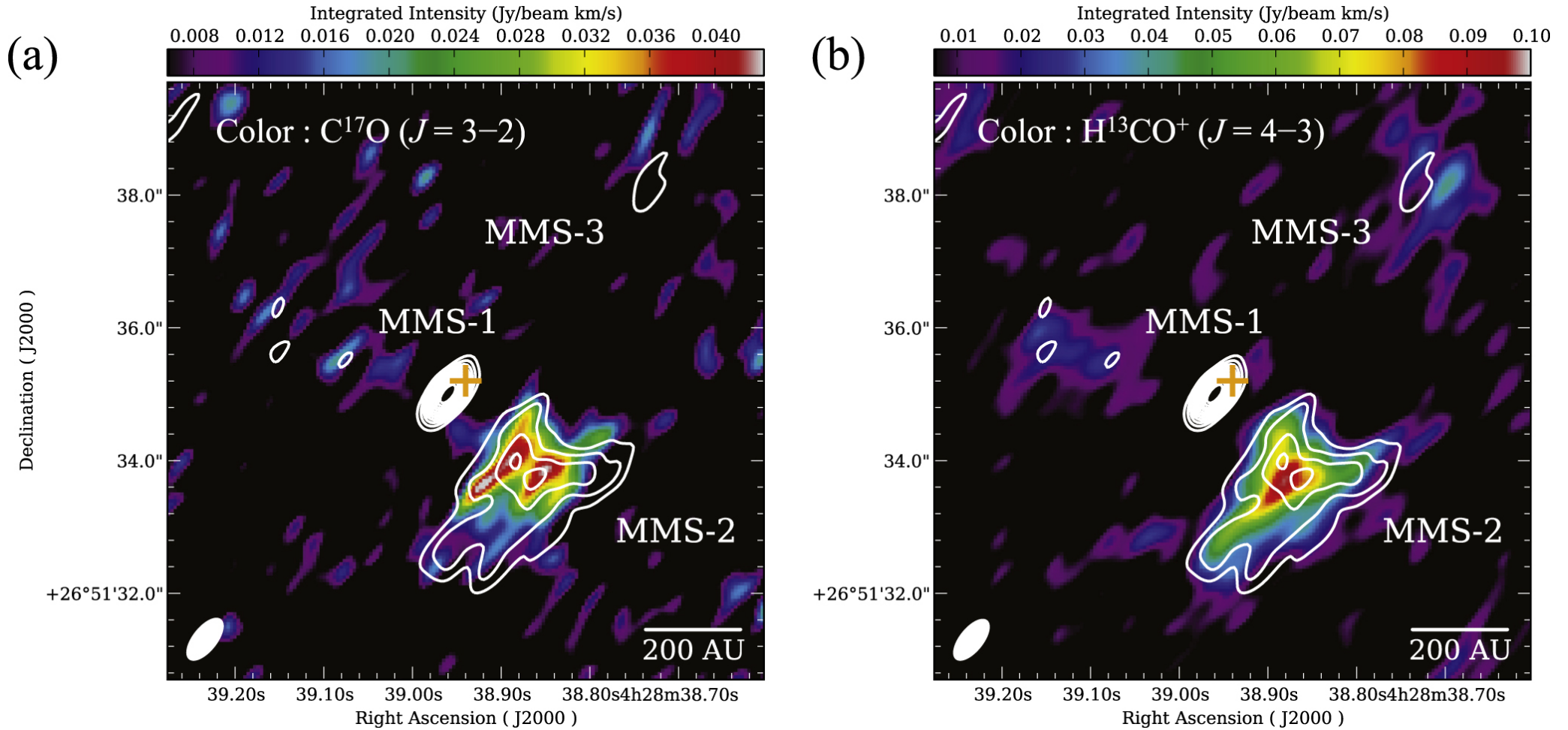
Figure 1. from REVEALING A DETAILED MASS DISTRIBUTION OF A HIGH-DENSITY CORE MC27/L1521F IN TAURUS WITH ALMA null 2016 APJ 826 26 doi:10.3847/0004-637X/826/1/26 https://dx.doi.org/10.3847/0004-637X/826/1/26 © 2016. The American Astronomical Society. All rights reserved.
