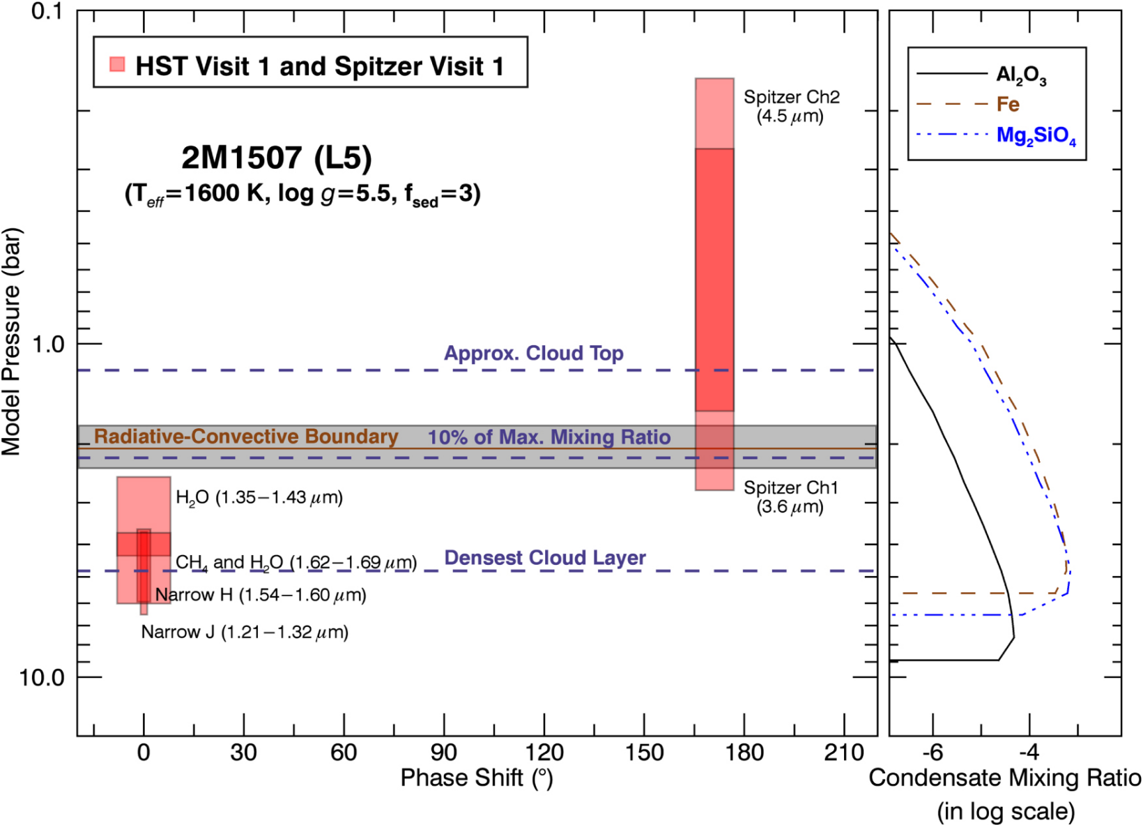
Figure 21. from EXTRASOLAR STORMS: PRESSURE-DEPENDENT CHANGES IN LIGHT-CURVE PHASE IN BROWN DWARFS FROM SIMULTANEOUS HST AND SPITZER OBSERVATIONS null 2016 APJ 826 8 doi:10.3847/0004-637X/826/1/8 https://dx.doi.org/10.3847/0004-637X/826/1/8 © 2016. The American Astronomical Society. All rights reserved.
