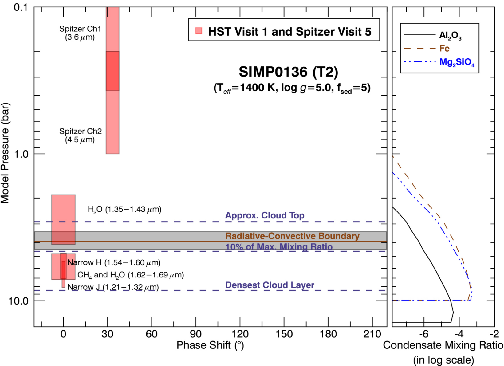
Figure 20. from EXTRASOLAR STORMS: PRESSURE-DEPENDENT CHANGES IN LIGHT-CURVE PHASE IN BROWN DWARFS FROM SIMULTANEOUS HST AND SPITZER OBSERVATIONS null 2016 APJ 826 8 doi:10.3847/0004-637X/826/1/8 https://dx.doi.org/10.3847/0004-637X/826/1/8 © 2016. The American Astronomical Society. All rights reserved.
