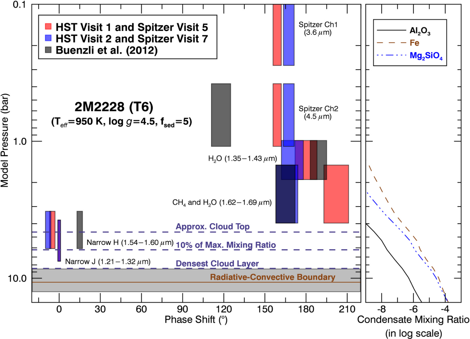
Figure 19. from EXTRASOLAR STORMS: PRESSURE-DEPENDENT CHANGES IN LIGHT-CURVE PHASE IN BROWN DWARFS FROM SIMULTANEOUS HST AND SPITZER OBSERVATIONS null 2016 APJ 826 8 doi:10.3847/0004-637X/826/1/8 https://dx.doi.org/10.3847/0004-637X/826/1/8 © 2016. The American Astronomical Society. All rights reserved.
