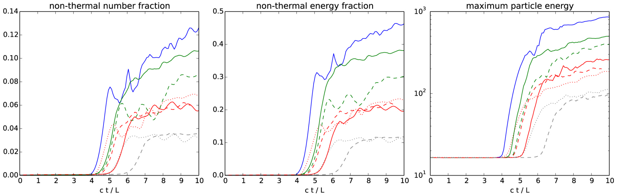
Figure 9. from KINETIC SIMULATIONS OF THE LOWEST-ORDER UNSTABLE MODE OF RELATIVISTIC MAGNETOSTATIC EQUILIBRIA null 2016 APJ 826 115 doi:10.3847/0004-637X/826/2/115 https://dx.doi.org/10.3847/0004-637X/826/2/115 © 2016. The American Astronomical Society. All rights reserved.
