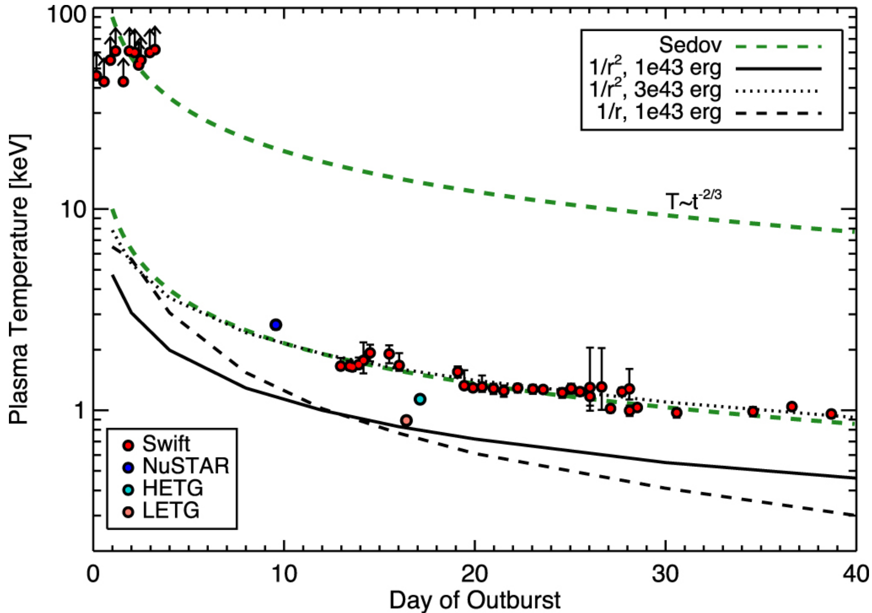
Figure 8. from COLLIMATION AND ASYMMETRY OF THE HOT BLAST WAVE FROM THE RECURRENT NOVA V745 Sco null 2016 APJ 825 95 doi:10.3847/0004-637X/825/2/95 https://dx.doi.org/10.3847/0004-637X/825/2/95 © 2016. The American Astronomical Society. All rights reserved.
