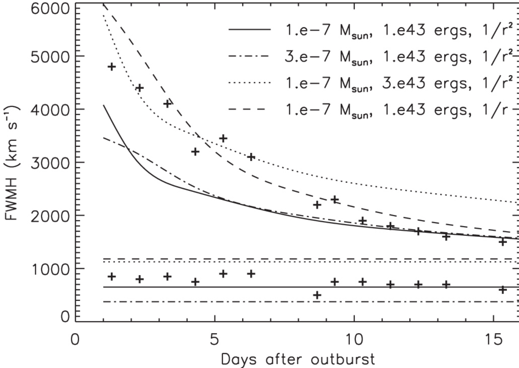
Figure 7. from COLLIMATION AND ASYMMETRY OF THE HOT BLAST WAVE FROM THE RECURRENT NOVA V745 Sco null 2016 APJ 825 95 doi:10.3847/0004-637X/825/2/95 https://dx.doi.org/10.3847/0004-637X/825/2/95 © 2016. The American Astronomical Society. All rights reserved.
