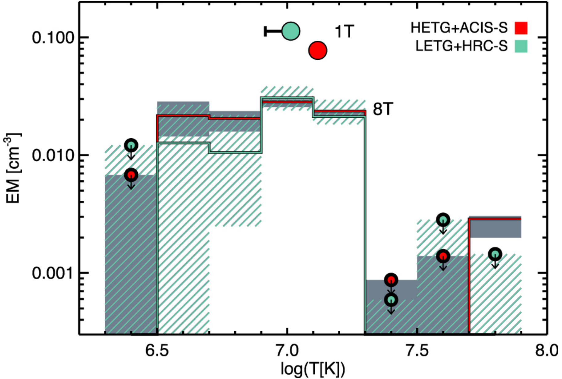
Figure 5. from COLLIMATION AND ASYMMETRY OF THE HOT BLAST WAVE FROM THE RECURRENT NOVA V745 Sco null 2016 APJ 825 95 doi:10.3847/0004-637X/825/2/95 https://dx.doi.org/10.3847/0004-637X/825/2/95 © 2016. The American Astronomical Society. All rights reserved.
