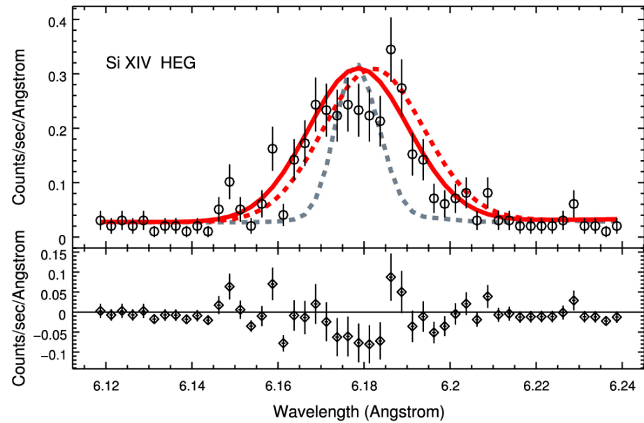
Figure 4. from COLLIMATION AND ASYMMETRY OF THE HOT BLAST WAVE FROM THE RECURRENT NOVA V745 Sco null 2016 APJ 825 95 doi:10.3847/0004-637X/825/2/95 https://dx.doi.org/10.3847/0004-637X/825/2/95
