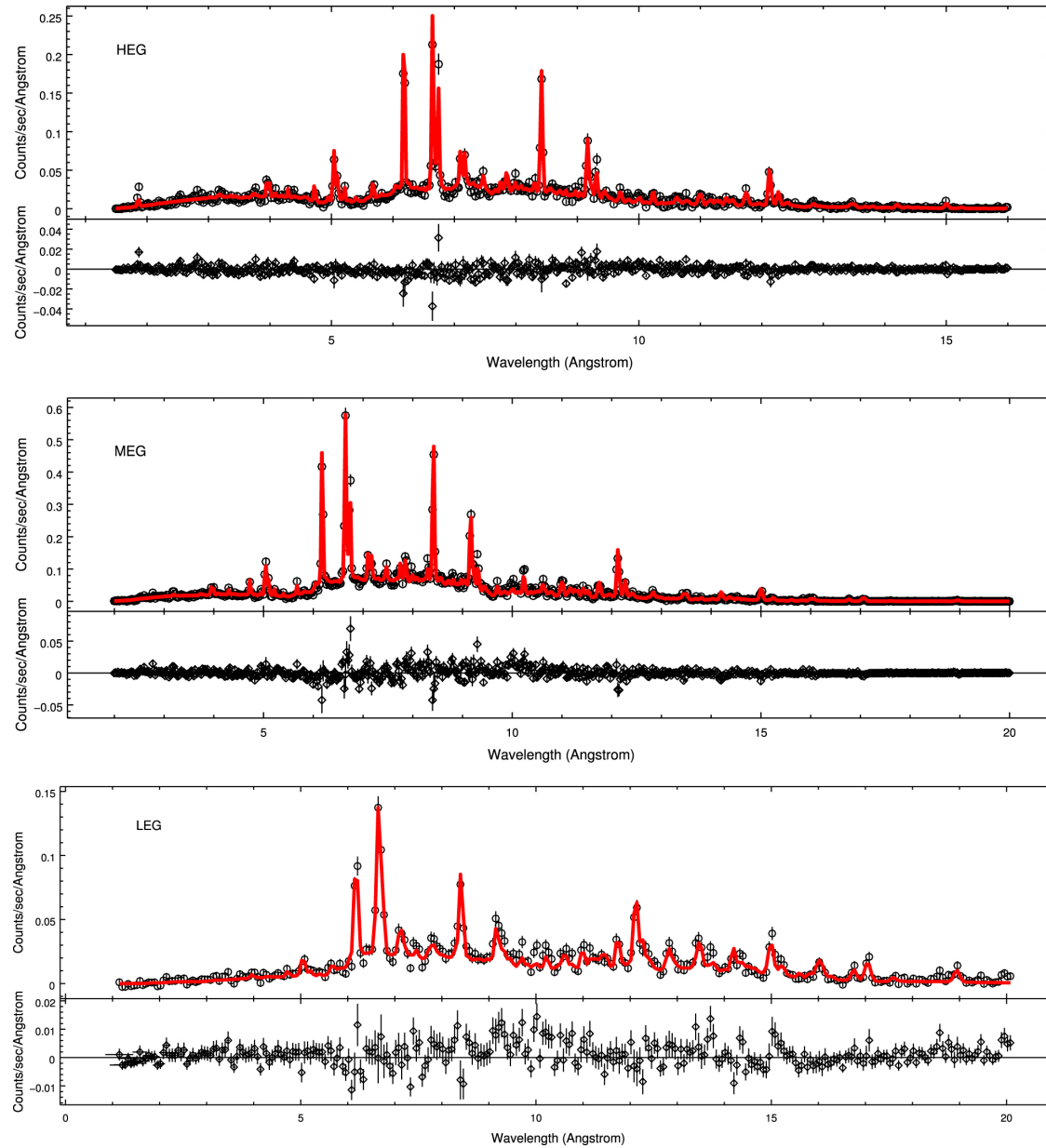
Figure 3. from COLLIMATION AND ASYMMETRY OF THE HOT BLAST WAVE FROM THE RECURRENT NOVA V745 Sco null 2016 APJ 825 95 doi:10.3847/0004-637X/825/2/95 https://dx.doi.org/10.3847/0004-637X/825/2/95 © 2016. The American Astronomical Society. All rights reserved.
