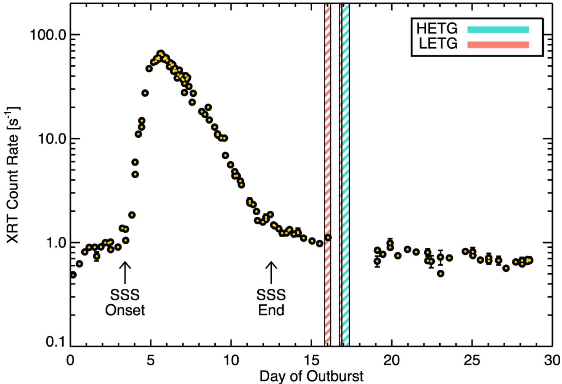
Figure 1. from COLLIMATION AND ASYMMETRY OF THE HOT BLAST WAVE FROM THE RECURRENT NOVA V745 Sco null 2016 APJ 825 95 doi:10.3847/0004-637X/825/2/95 https://dx.doi.org/10.3847/0004-637X/825/2/95 © 2016. The American Astronomical Society. All rights reserved.
