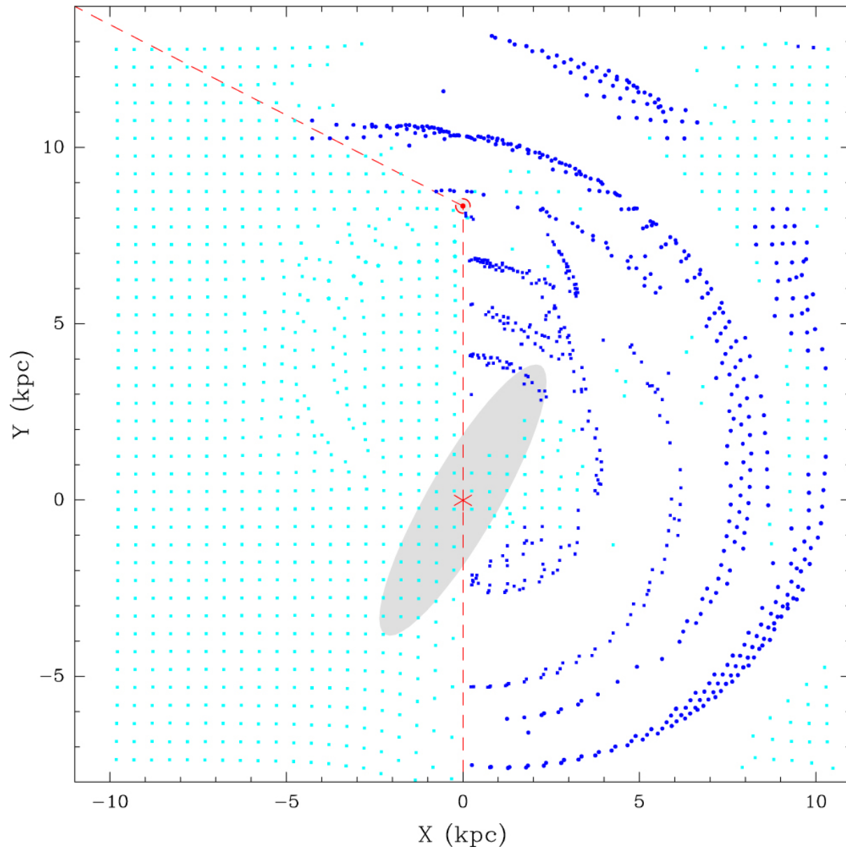
Figure 6. from A PARALLAX-BASED DISTANCE ESTIMATOR FOR SPIRAL ARM SOURCES null 2016 APJ 823 77 doi:10.3847/0004-637X/823/2/77 https://dx.doi.org/10.3847/0004-637X/823/2/77 © 2016. The American Astronomical Society. All rights reserved.
